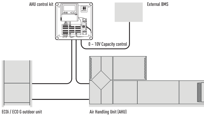
ECOi / ECO G outdoor unit Air Handling Unit (AHU) Demand control on the outdoor unit managed by external 0-10 V signal.
