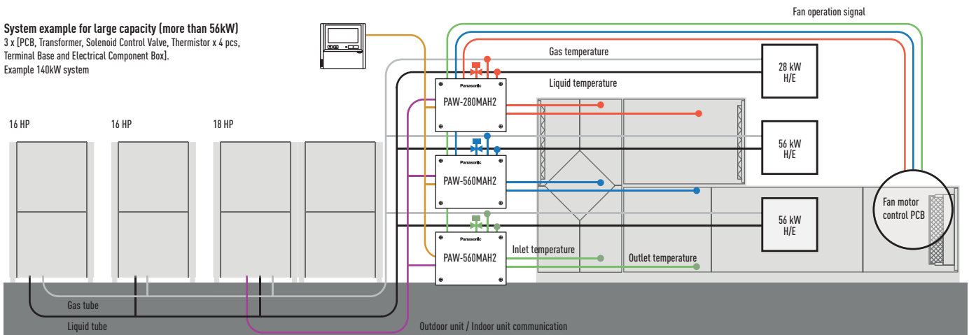
ECOi / ECO G outdoor unit Air Handling Unit (AHU) Demand control on the outdoor unit managed by external 0-10 V signal.
